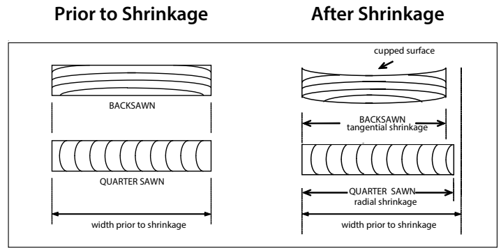
Figure 2. - Relative cupping in backsawn & quarter sawn.
